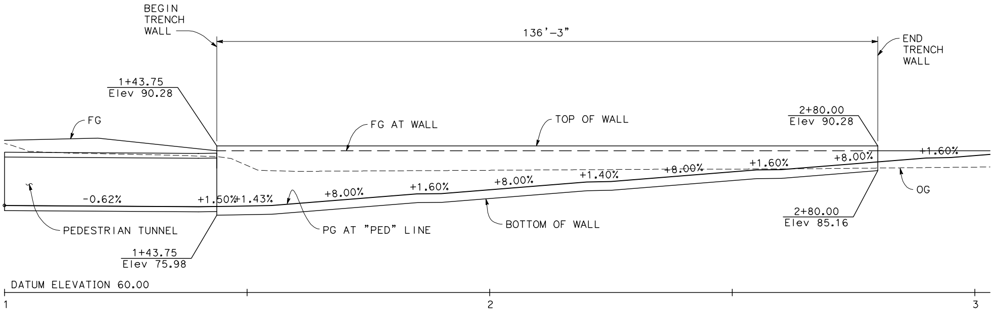
DEVELOPED ELEVATION
