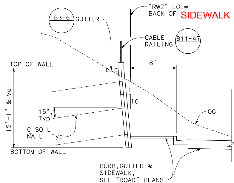
TYPICAL SECTION 1" = 5'
