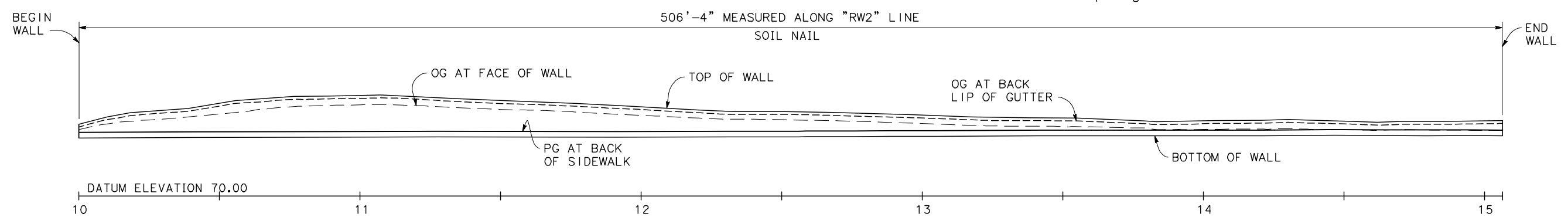
ELEVATION 1" = 20'
